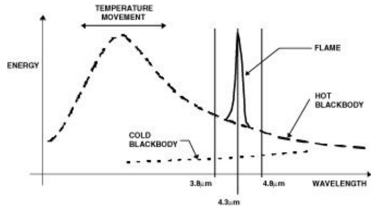
Fig. 3. Blackbody Rejection
