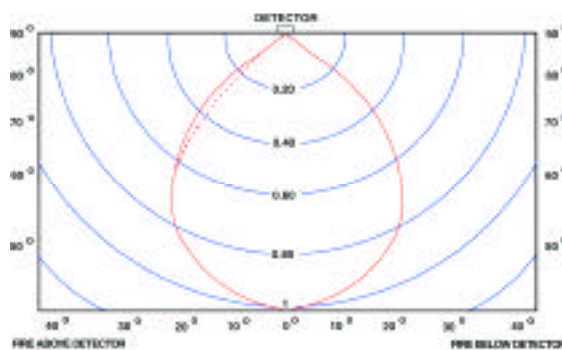
Figure 2b - Pan Fires- Relative Range vs Angle of Incidence. Vertical Dotted Line Shows Flameproof Version with Steel Guard Fitted Solid Lines Shows IS Version
