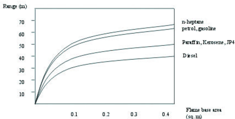
Fig. 1 - Fire Range Test Data
